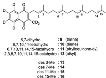
Figure 6. Compounds used in SAR study of SXR.
