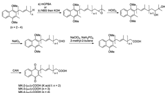
Figure 17. Synthesis of MK- n -( \omega -2)-COOH derivatives (Fujii et al.).
