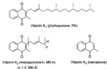
Figure 1. Structures of vitamin K homologues.
