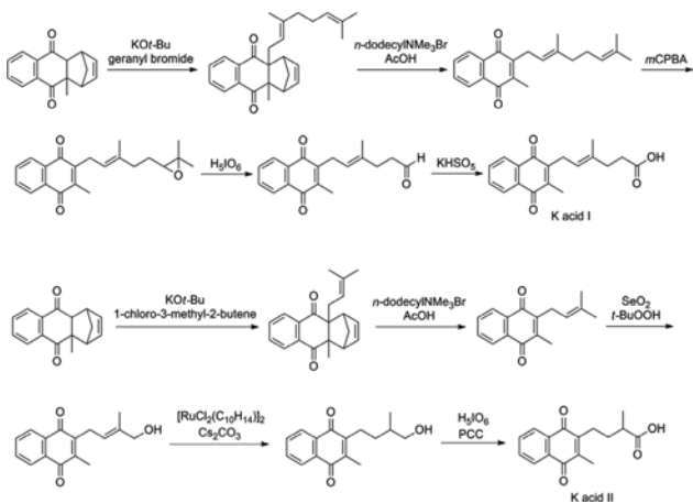
Figure 12. Synthetic routes of K acid I and K acid II (Teitelbaum et al.).
