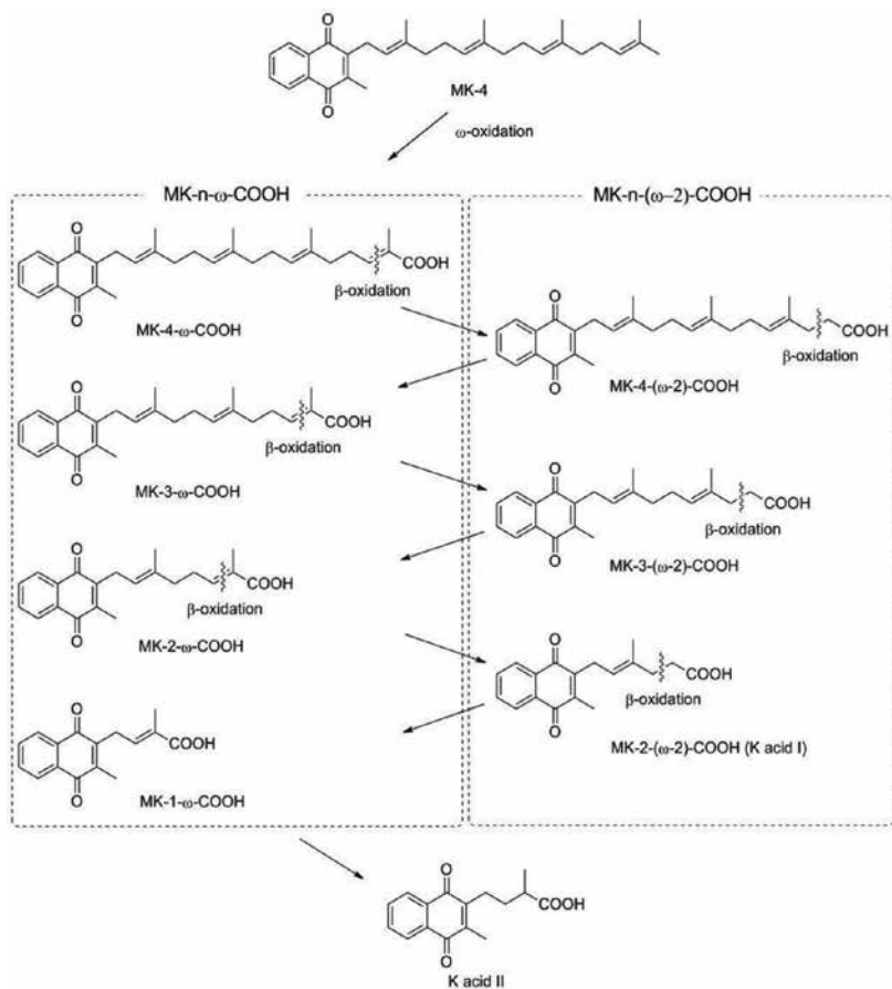
Figure 9. Putative catabolic pathways of MK-4.
