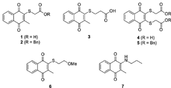
Figure 4. Examples of side chain-modified Cpd 5 derivatives.
