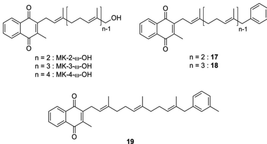
Figure 8. Structures of menaquinone derivatives with modified terminal.
