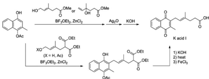
Figure 10. Synthetic route to K acid I (Watanabe et al.).
