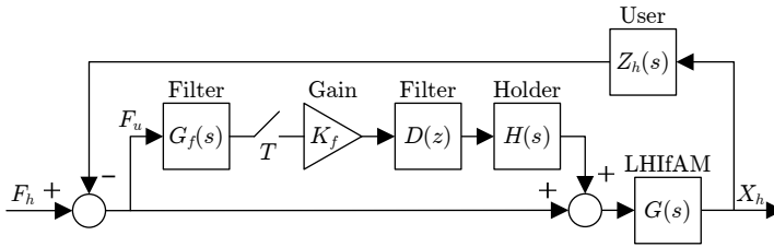
Fig. 24. Final force feedforward strategy with digital filter.
