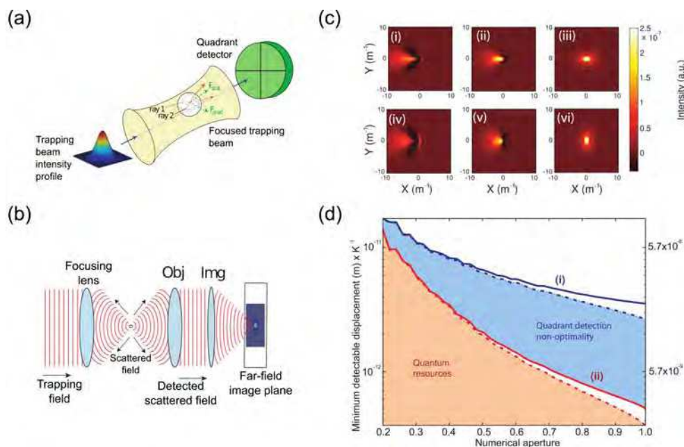
Fig. 7. (a) Illustration showing a TEM 00 trapping field focused onto a spherical scattering particle. The gradient and scattering forces are given by F_{\text{grad}} and F_{\text{scat}} , respectively. (b) Schematic representation of the trapping and scattered fields in an optical tweezers. The trapping field is incident from the left of the diagram. Obj: objective lens, and Img: imaging lens. (c) Interference pattern of the trapping and forward scattered fields in the far-field plane. Figures (i)-(iii) and (iv)-(vi) assume that the trapping field is x - and y -linearly polarised, respectively. The particle displacements are given by (i), (iv): 1 \mu\text{m} ; (ii), (v): 0.5 \mu\text{m} ; and (iii), (vi): 0 \mu\text{m} . (d) Minimum detectable displacement normalised by K , versus collection lens NA for (i) split and (ii) spatial homodyne detection. The solid and dashed lines are for x - and y -linearly polarised trapping fields, respectively. The axis on the right shows the minimum detectable displacement assuming 200 mW trapping field power, \lambda = 1064 \text{ nm} , particle radius a = 0.1 \mu\text{m} , permittivity of the medium \epsilon_1 = 1 , permittivity of the particle \epsilon_1 = 3.8 and trapping field focus of 4 \mu\text{m} . Absorptive losses in the sample were assumed to be negligible. Figures (b), (c) and (d) were reproduced from Tay et al. (2009), with permission.
