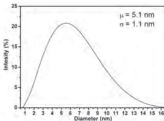
Fig. 5. Ligand-stabilized AgNPs diameter distribution by DLS.
