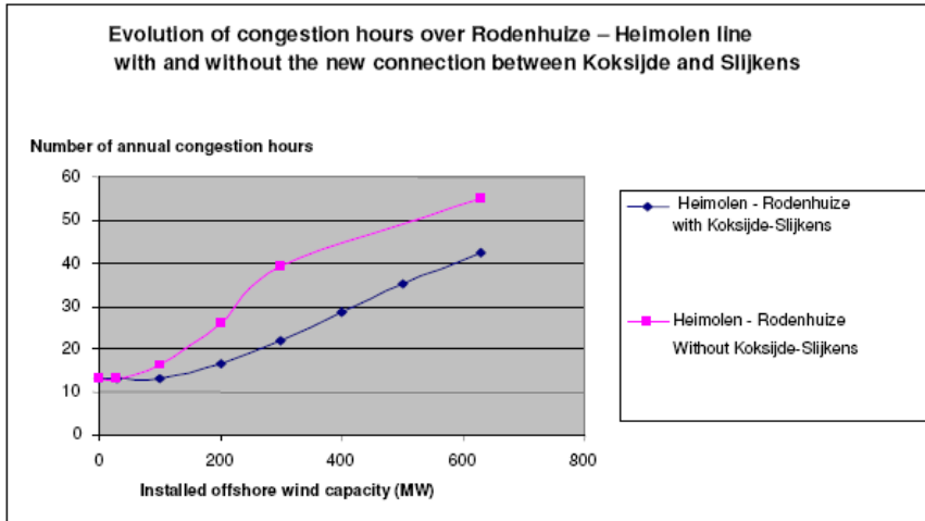
Fig. 12. Evolution of congestion hours between Rodenhuize and Heimolen with and without the added connection Koksijde-Slijkens (importation level of 1 GW and 630 MW installed offshore wind power)
