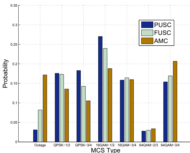
Fig. 9. MCS distribution for PUSC/FUSC/AMC with beamforming.
