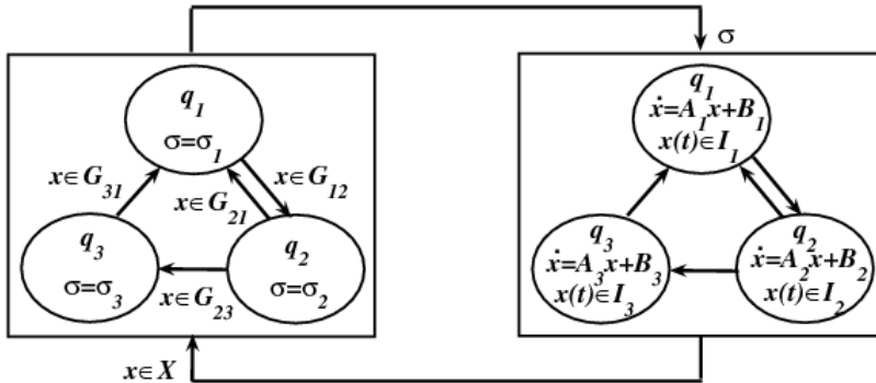
Fig. 3. Hybrid description of a conventional boost converter under CCM and DCM (Sreekumar & Agarwal, 2008).
