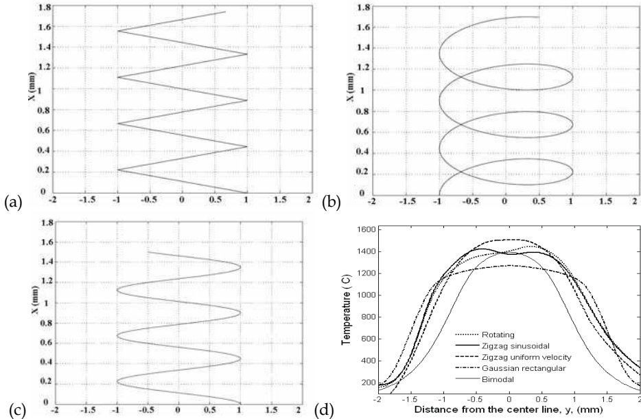
Fig. 6. (a) dithering beam with uniform velocity (b) rotating beam (c) dithering beam with sinusoidal velocities (d) Variation of the maximum temperature rise with the distance from the center line, y , for different moving patterns.
