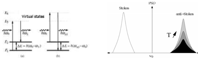
Fig. 4. Origin of Raman scattering (left) and sensitivity to temperature (right). “PSD” stands for power spectral density.
