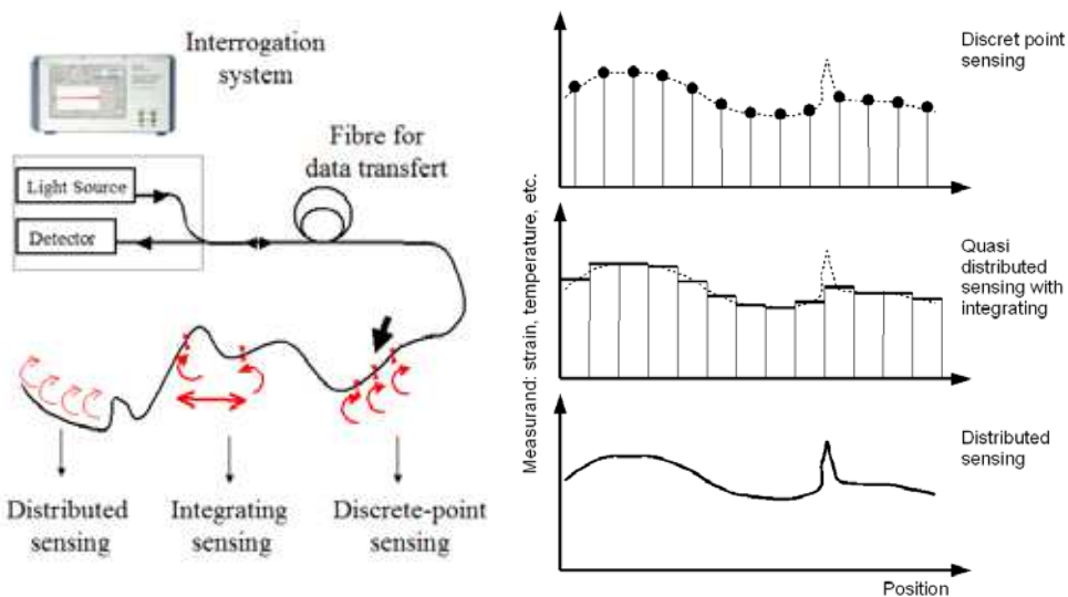
Fig. 1. Concepts of point, integrating and distributed sensing.
