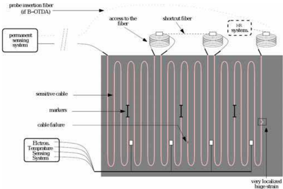
Fig. 15. Modern instrumentation scheme for SHM applications.
