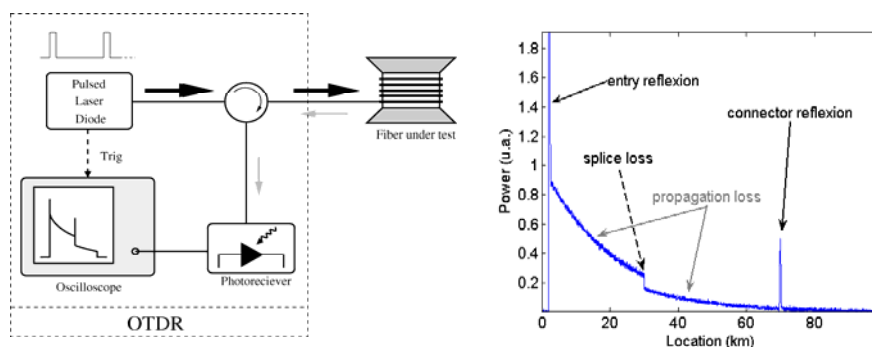
Fig. 3. OTDR (Optical Time Domain Reflectometry) operating principle, and typical trace.
