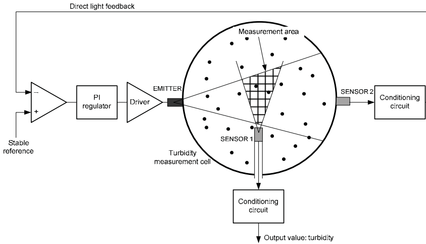
Fig. 6. Three-beam feedback turbidimeter. The sensor 1 conditioning circuit output contains the turbidity information.
