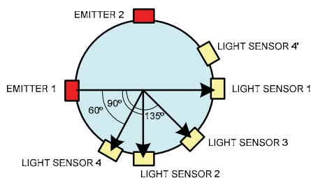
Fig. 3. Two-phases multi-beam turbidimeter.
