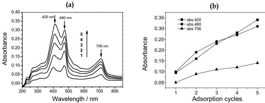
Fig. 9. Evolution of the spectrum as a multilayer film of PDDA + /TSPP - that was deposited onto a 200 μm core diameter multimode optical fibre with a stripped silica core of 1 cm: (a) absorbance spectra (derived from the transmission spectra using eq. (2)); (b) absorbance change due to film deposition monitored at wavelengths of 420 nm (squares), 480 nm (circles), and 706 nm (triangles).
