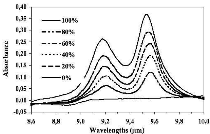
Fig. 1. Absorbance spectrum of the different concentration of ethanol in water measured in the infrared spectral range of 8.6–10 μm (Le Coq et al., 2002)
