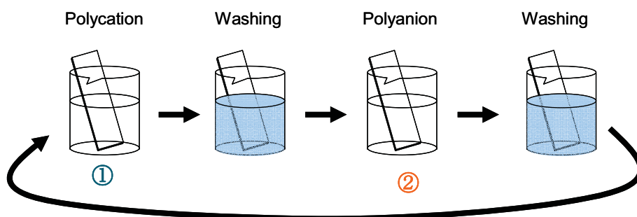
Fig. 2. Schematic illustration of the layer-by-layer (LbL) method
