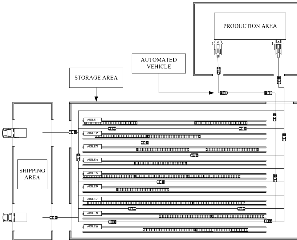
Fig. 4. Plant layout.
