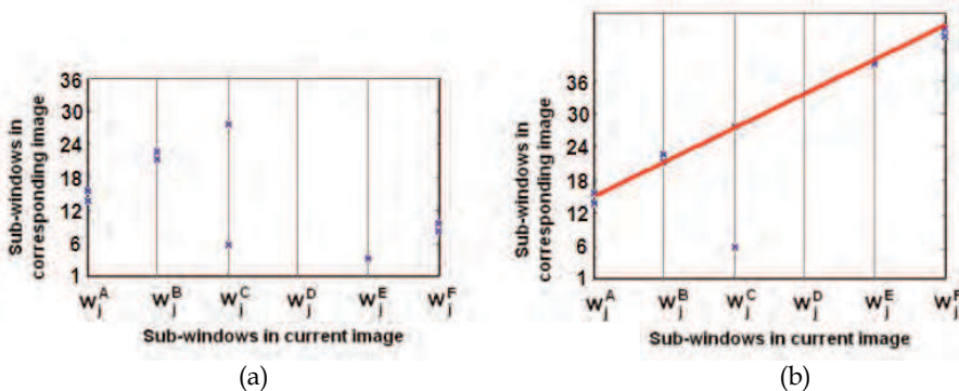
Figure 10. Computing the steering speed of the robot with the sub-windows approach. This speed is proportional to the ordinate in the origin of the fitted line
