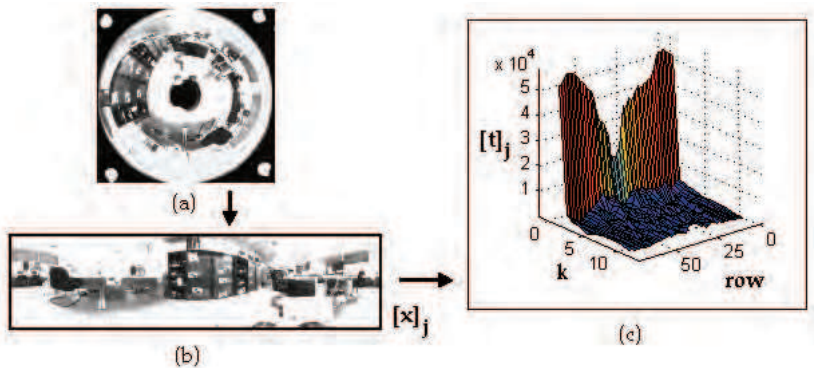
Figure 7. For each point on the route, the omnidirectional view (a) is transformed into the panoramic view (b). Then, the Fourier transform is computed row to row (c). The main information is in the module of the components of lower frequency so these components are retained in a matrix that identifies that point of the route
