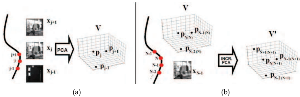
Figure 5. (a) Using PCA, the images of the route are dimensionally reduced. (b) Input and output data of the Incremental PCA process in each iteration. When a new image arrives, the projections in the database and the matrix V are updated
