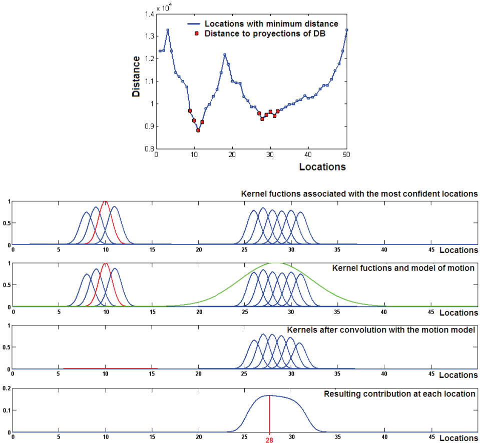
Figure 8. Improvement of the localization phase through a probabilistic-based approach. The new location depends on the previous one and the image acquired
