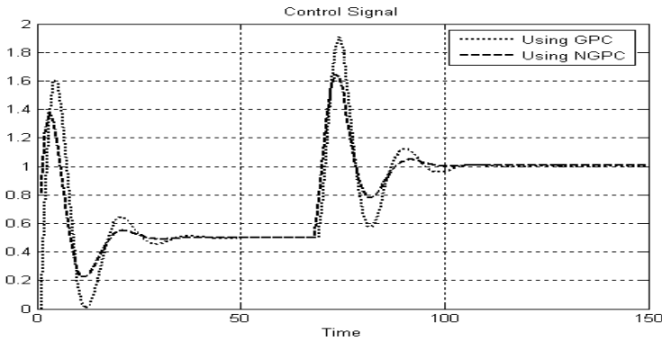
Fig. 7. Control Signal for System I
