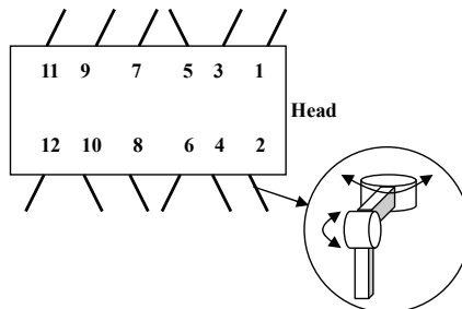
Figure 6. Multi-legged robot (Ito & Matsuno, 2002)
