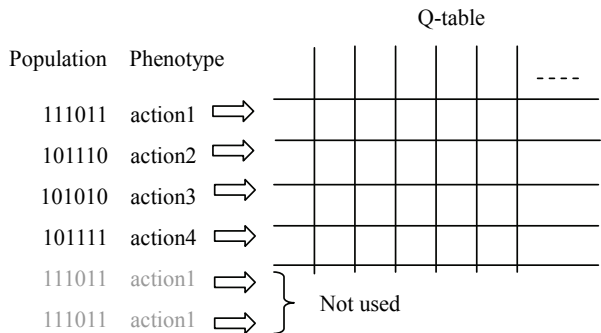
Figure 2. Q-table created from a set of individuals (Ito & Matsuno, 2002)
