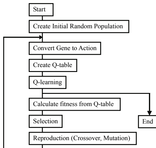
Figure 1. Outline of QDSEGA (Ito & Matsuno, 2002)
