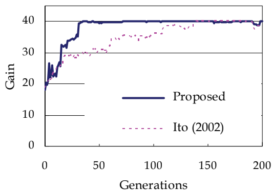
Figure 7. Average gain over the generation
