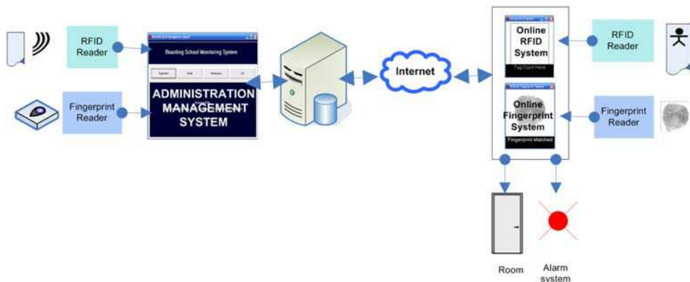
Fig. 2. BoSs Architecture
