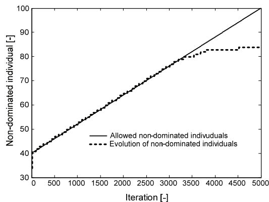
Figure 7. Evolution of non-dominated individuals along iterations
