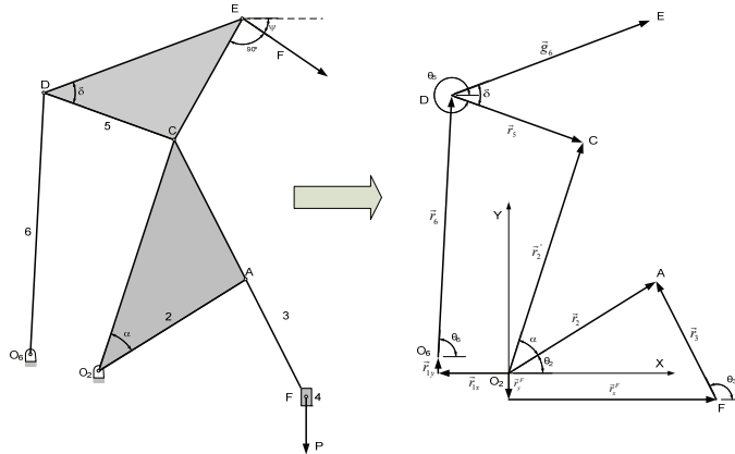
Figure 5. Kinematic study of the mechanism
