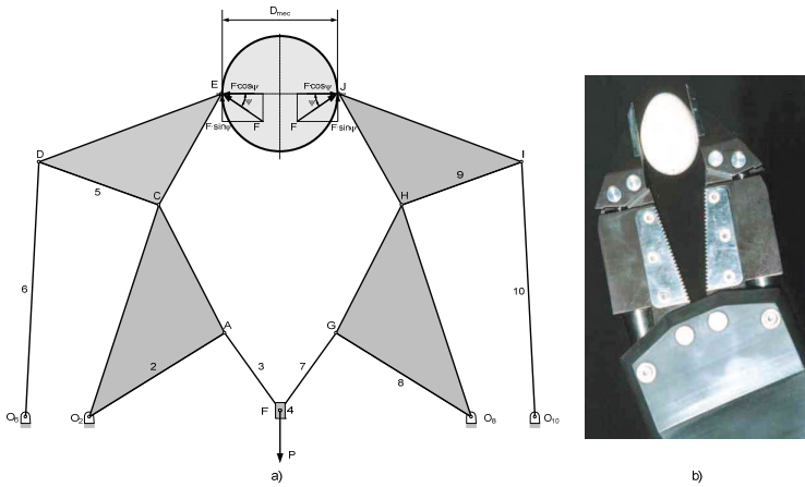
Figure 4. a) Hand robot mechanism for problem 1 and 2. b) Real robot manipulator
