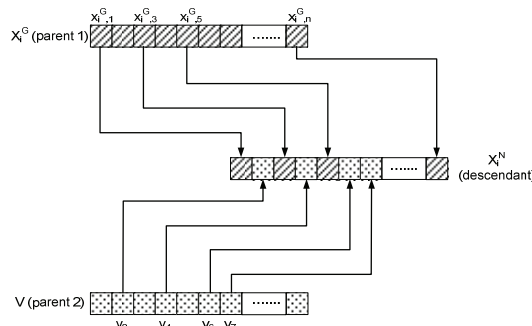
Figure 1. Reproduction scheme based on discrete multipoint crossover
