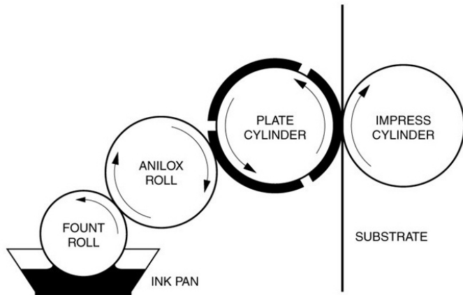
Fig. 4. Schematic representation of a flexographic press
