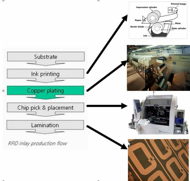
Fig. 14. Different steps of the plating process
