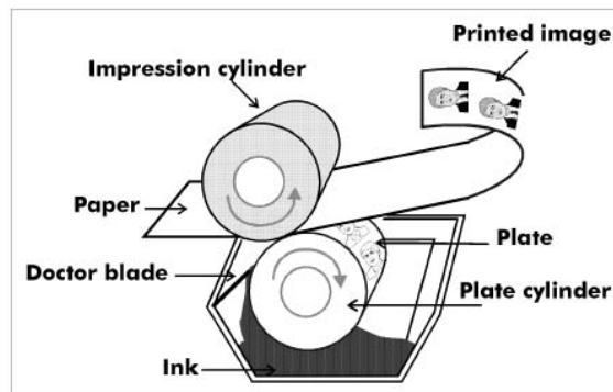
Fig. 7. Schematic representation of a rotogravure printer
