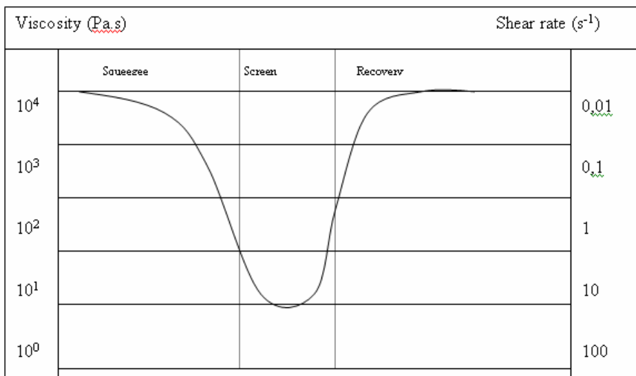
Fig. 8. Typical shear rates and viscosities during the screen print process
