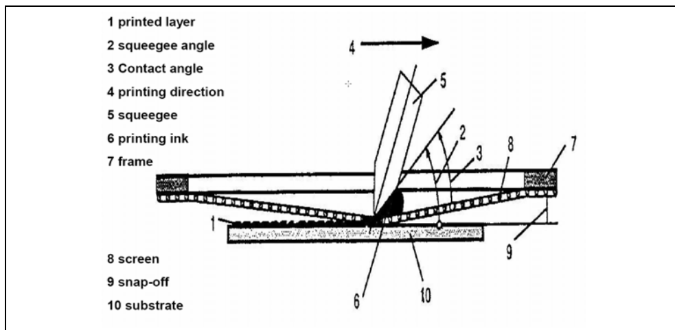
Fig. 3. Schematic figure of the screen printing process
