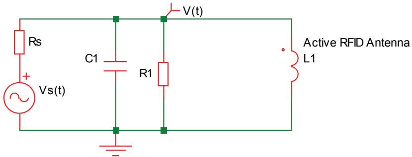
Active RFID's Equivalent circuit
