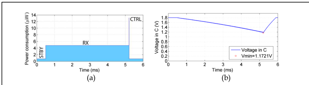
Fig. 16. Power distribution and supply voltage drop of the Select command for Tari = 25 \mu s and BLF = 240 \text{ kHz} .
