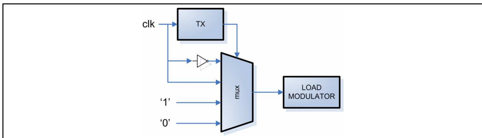
Fig. 5. Full- T_{pri} base transmitter.
