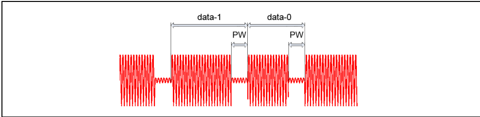
Fig. 9. Modulated RF signal during downlink communication.
