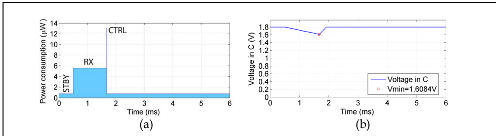
Fig. 15. Power distribution and supply voltage drop of the Select command for Tari = 6.25 \mu s and BLF = 240 \text{ kHz} .
