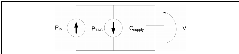
Fig. 11. Tag model receiving CW from the reader.
