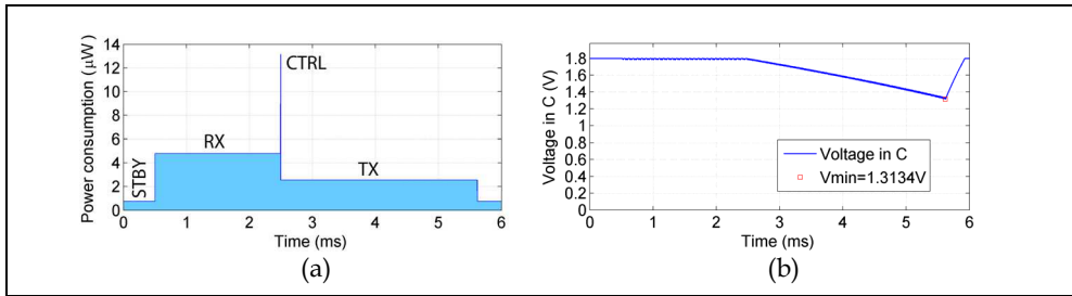
Fig. 13. Power distribution and voltage drop of a Read command for Tari = 25 \mu\text{s} and BLF = 40 \text{ kHz} .
