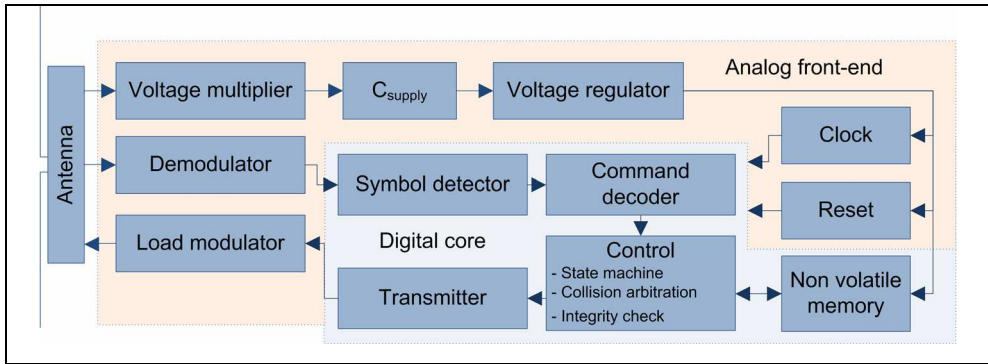
Fig. 1. Architecture of a passive RFID tag.
