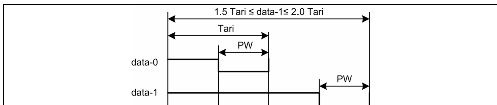
Fig. 3. PIE codification, from (EPC Global, 2005).
