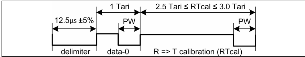
Fig. 4. Forward link calibration in the preamble, from (EPC Global, 2005).
