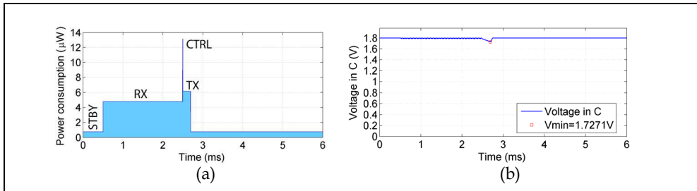
Fig. 14. Power distribution and supply voltage drop of the Read command for Tari = 25 \mu s and BLF = 640 \text{ kHz} .
