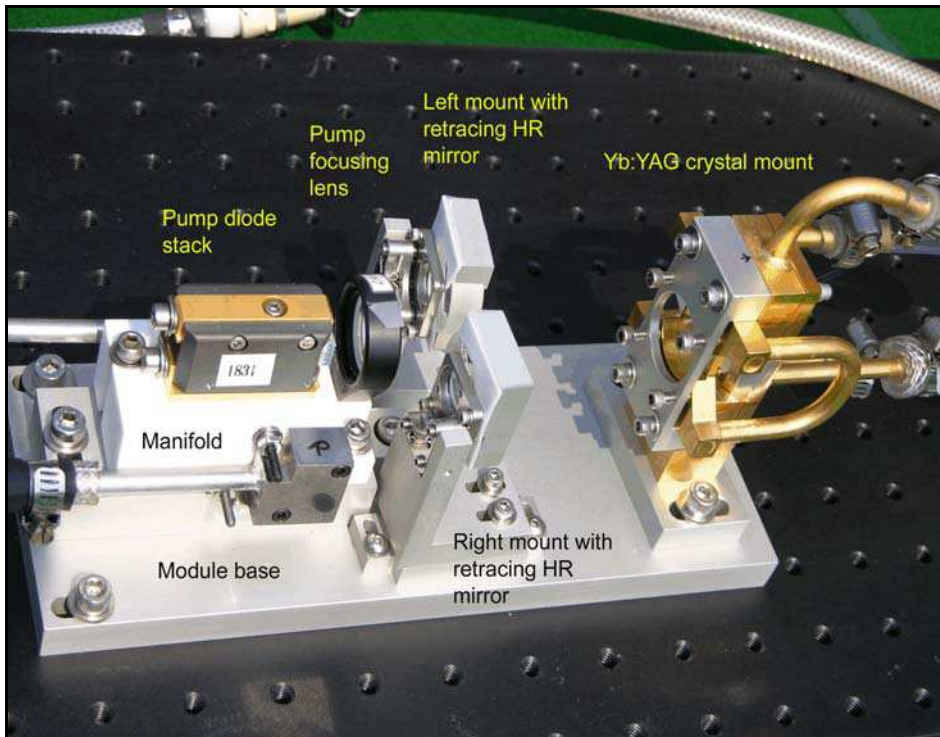
Fig. 6. View of the assembled Yb:YAG gain module
