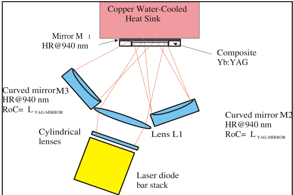
Fig. 3. Multi-pass pumping scheme of Yb:YAG laser
