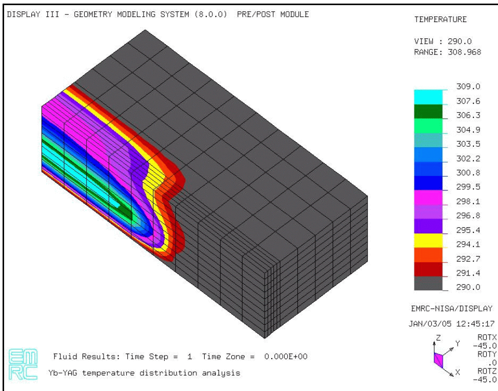
Fig. 2. Temperature distribution in composite 3%Yb:YAG crystal of 3 x 10 x 21.6 mm with homogeneous absorbed pump light area of 1.5 x 1.5 x 10.8 mm, which is cooled from the bottom and from the top faces, except window of 0.22 x 13 mm. Maximum heat power generation in crystal is 20 W. Because of symmetry, only one fourth of the crystal is shown.
