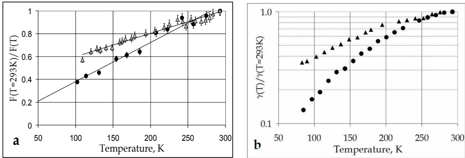
Fig. 12. Temperature dependence of the focal length of thermal lens F (a) and depolarization \gamma in the TGG with the [001] orientation (circles, F(T=293K)=191\text{cm} , \gamma(T=293K)=5.2\cdot 10^{-3} ) and in glass MOC-04 (triangles, F(T=293K)=581\text{cm} , \gamma(T=293K)=5.1\cdot 10^{-3} ).
