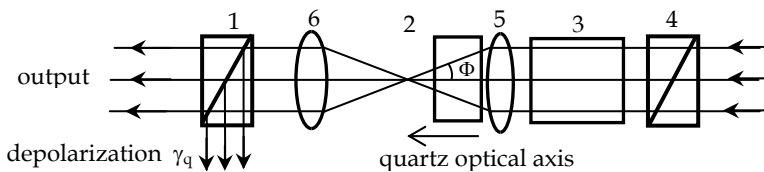
Fig. 7. Depolarization compensation in FI: 1,4 – polarizers, 2 – 45° QR, 3 – MOE, 5 and 6 – lenses of telescope. MOE and QR rotate in opposite directions.
