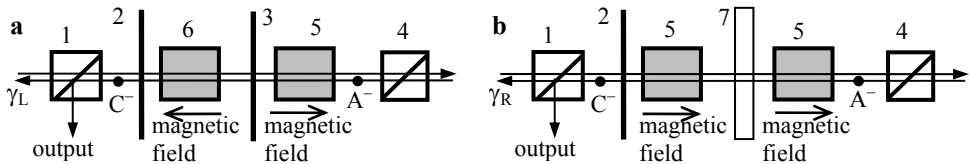
Fig. 9. FI designs with a \lambda/2 plate (a) and QR (b) (Khazanov, 1999). 1,4 - polarizers, 2,3 - \lambda/2 plates, 5 - 22.5^\circ MOE rotating clockwise, 6 - 22.5^\circ MOE rotating anticlockwise, 7 - 67.5^\circ QR.
