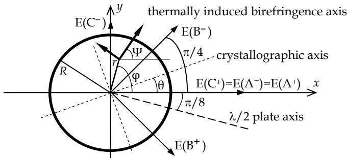
Fig. 2. Cross-section of magneto-optical crystal: r , \varphi are polar coordinates; \theta is angle of inclination of the crystallographic axis; \Psi is angle of inclination of eigen polarization of thermally induced birefringence.
