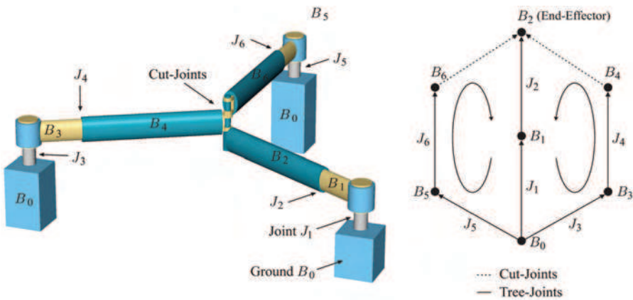
Figure 3. Topological graph, and spanning tree of the RP/2RPR manipulator.
