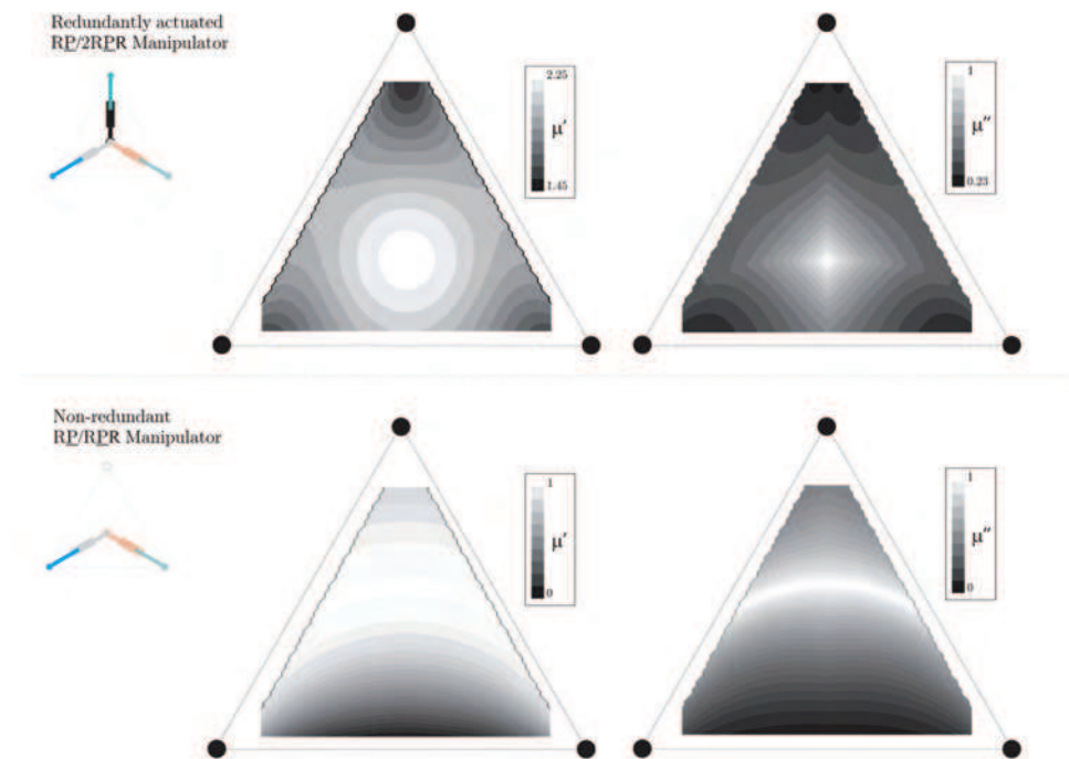
Figure 2. Manipulability distribution for the redundantly actuated RP/2RPR and the non-redundant RP/RPR manipulator.
