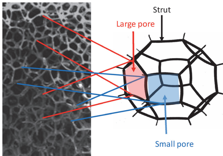
Figure 3. SEM pictures of two samples of polyurethane (PU) foam and the relationship with the derived model tetrakaidcahedron unit cell (Kelvin cell) of the PU structure (adapted from [44]). Notice the continuity of the cell microstructure across the figure that includes two samples.
