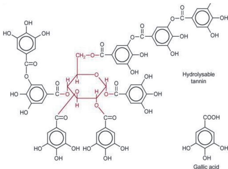
Figure 9. Hydrolysable tannins.
