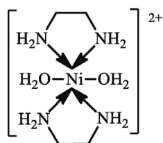
Figure 3. Structure of chelate with three ethylenediamine ligands.
