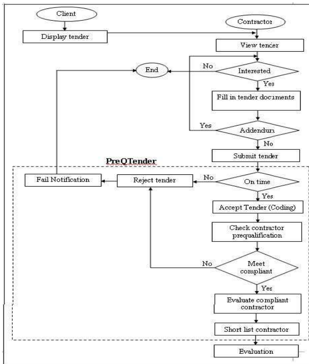
Fig. 1. Overall Workflow of PreQTender
