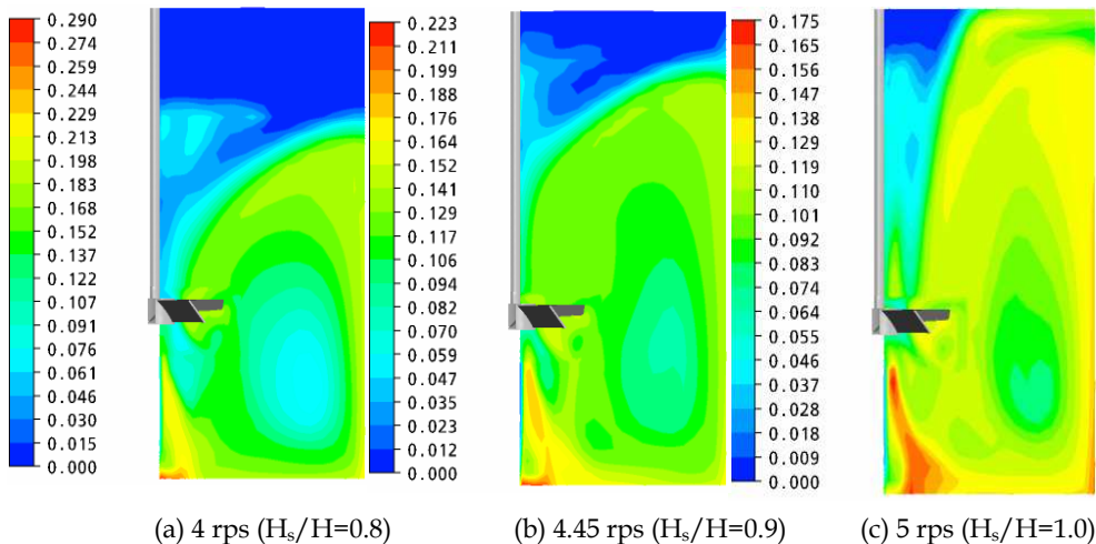
Fig. 4. Cloud height predicted by CFD simulation for PBTD impeller at different rotational speeds (particle size of 350 μm with solid loading of 10 vol. %)
