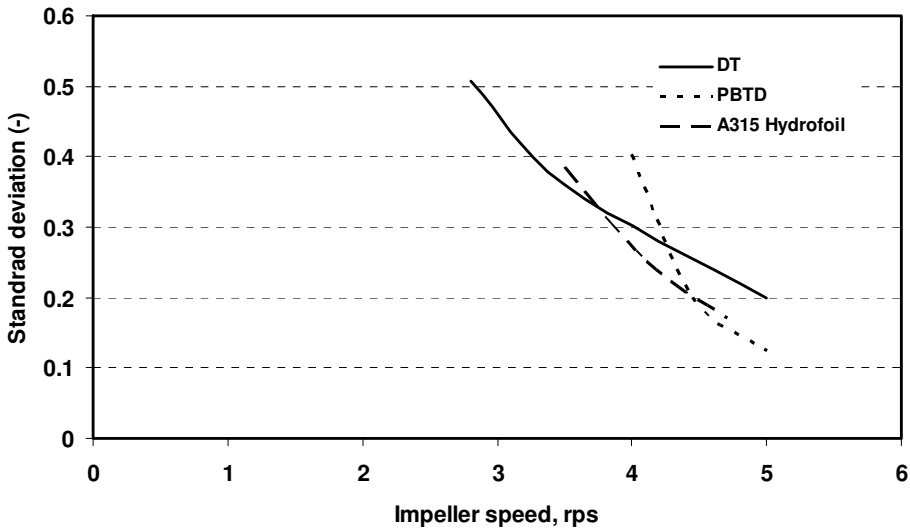
Fig. 3. Standard deviation values obtained from CFD with respect to impeller rotational speed for DT, PBTD and A315 hydrofoil impeller (particle size of 350 μm with solids loading of 10 vol. %)
