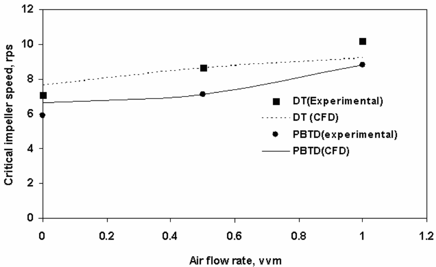
Fig. 9. Effect of air flow rate on Critical impeller speed for different impellers (particle size= 230 μm & particle loading = 30 wt %)
