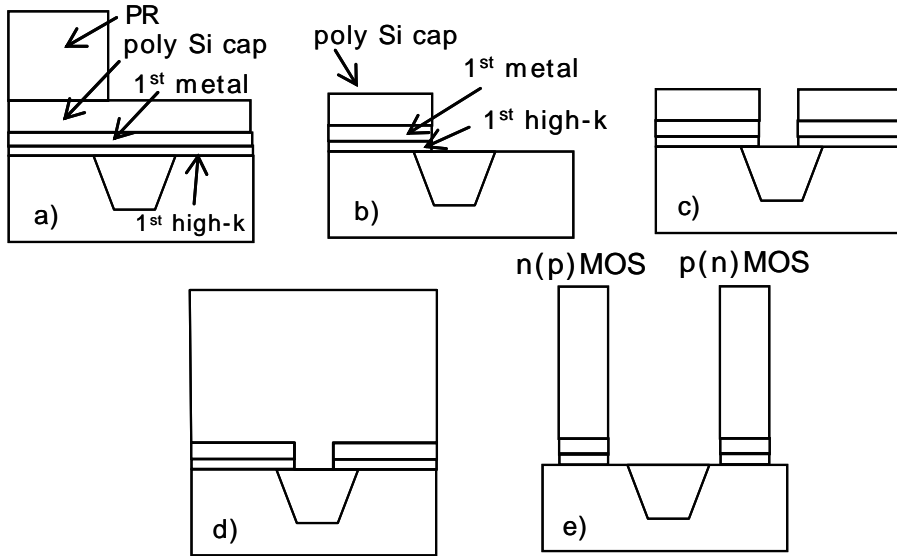
Fig. 4. Dual Metal Dual Dielectrics (DMDD) CMOS integration scheme
