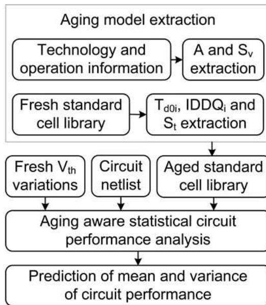
Fig. 10. Statistical circuit performance analysis flow.
