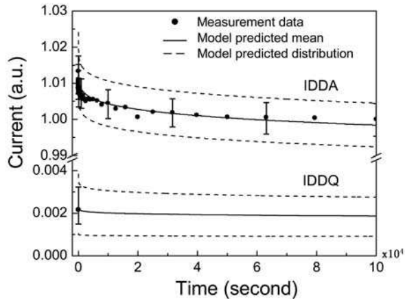
Fig. 13. The prediction of IDDA and IDDQ degradation.
