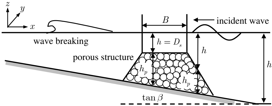
Fig. 1. Waves propagating over a submerged permeable structure.
