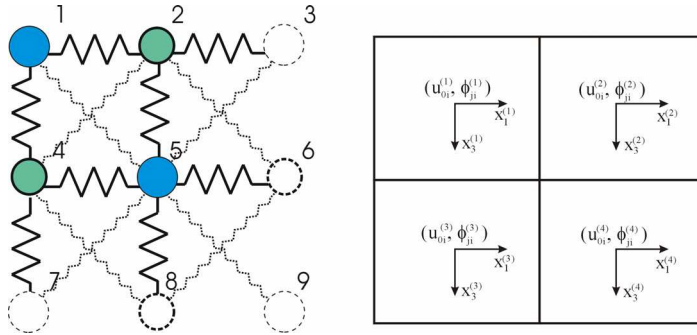
Fig. 4. Representative unit cell and the equivalent continuum
