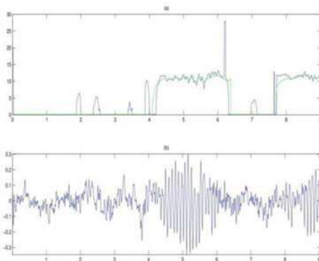
Fig. 5. (a) Instantaneous Frequency using the Kalman Smoother and EM (green line) and the Kalman Smoother only (blue line) (b) Trial data.
