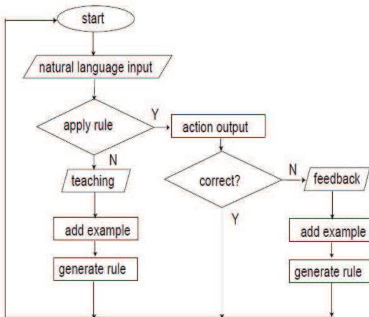
Fig. 7. System flowchart
