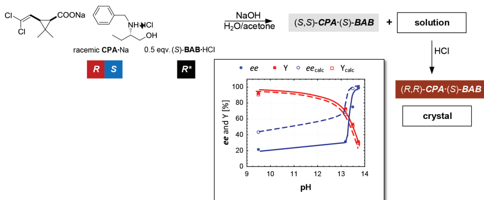
Figure 1. pH-dependent resolution of racemic cis -permethric acid with ( S )- N -benzyl-2-aminobutanol.
