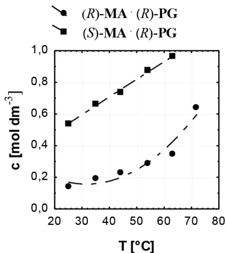
Figure 12. Temperature-dependent solubility of (S)-MA·(R)-PG and (R)-MA·(R)-PG diastereomers.
