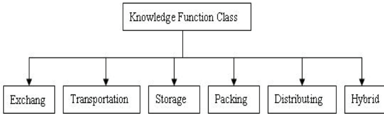
Fig. 6. Function category
