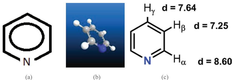
Figure 1. (a) The double bonds in pyridine are shared between all of the atoms in the circle so that they can be drawn as a circle instead of individual bonds. (b) Pyridine. (c) The hydrogen atoms on pyridine have three distinct chemical shifts. Pyridine shares the electrons in the entire circle, but the nitrogen draws more electrons to it, causing a slight dipole to form.
