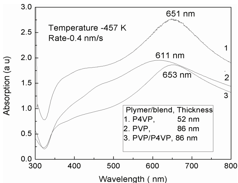
Figure 2. Optical absorption spectra of P4VP, PVP, and their composite.
