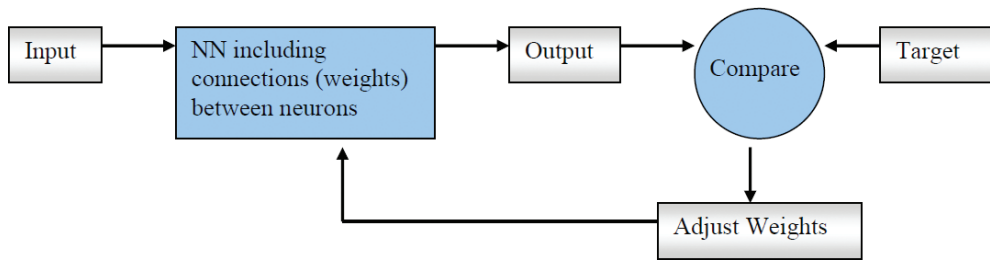
Figure 4. Description of BPNN training the data sets [29].
