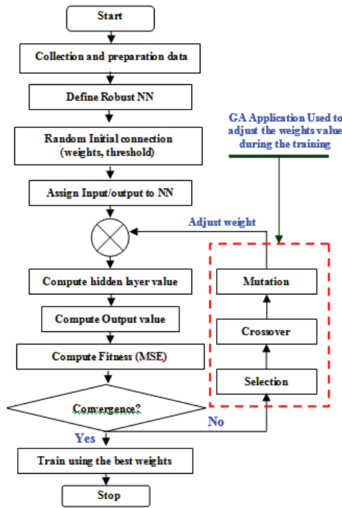
Figure 5. Neuro-genetic algorithm in BPNN development [35].
