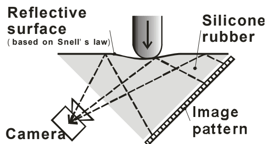
Fig. 8. Reflection type tactile sensor (Saga, et al. 2007)
