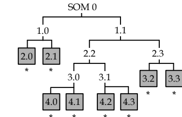
(c) Hierarchical learning with SOM.
