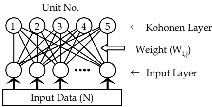
(a) Structure of SOM.
