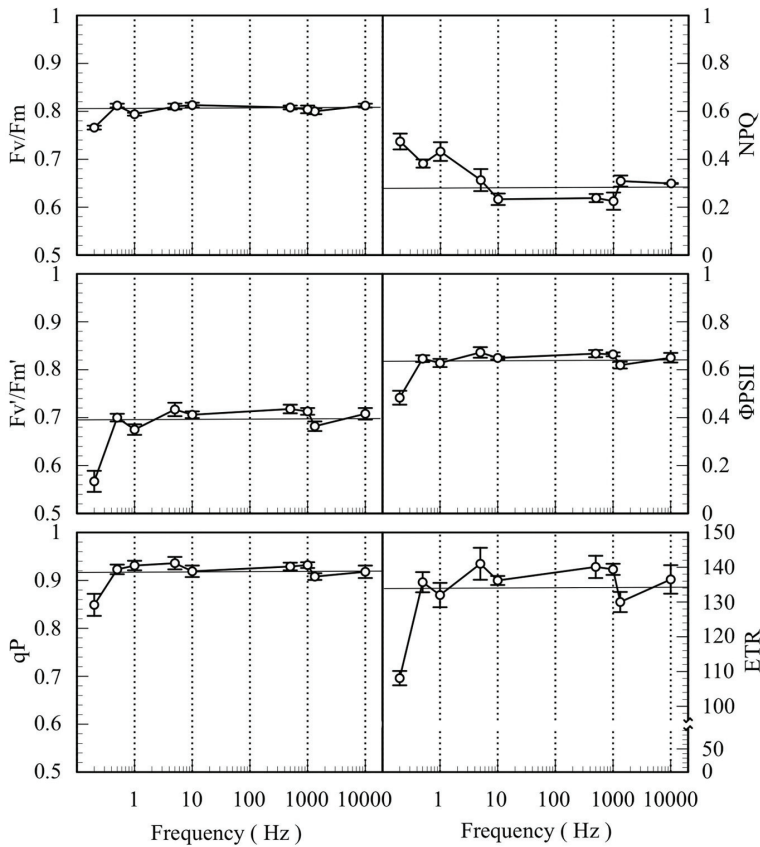
Figure 7. Chlorophyll fluorescent parameters of leaves grown under non-pulsed continuous lighting (horizontal line) and under different pulsed lighting cycles (○). Fv/Fm and Fv'/Fm' were measured with dark-adapted or exposing leaves to 500 \mu\text{mol m}^{-2} \text{s}^{-1} PPFD (saturated irradiance with or without pulse cycles) to estimate photochemical (qP) and non-photochemical (NPQ) quenching.
