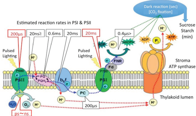
Figure 9. Photochemical reactions of photosynthesis are connected by an electron transport chain (ETC) between Photosystem I (PSI) and II (PSII), and ATP synthase embedded in thylakoid membrane in chloroplast. ETC composes of PSII reaction center (P680), plastiquinone (PQ), cytochrome b 6 f complex ( b 6 f ), plastocyanin (PC), PSI reaction center (P700), ferredoxin (Fd), ferredoxin-NADP + reductase (FNR). Each estimated electron transfer rate is an example from Refs. [3, 4].
