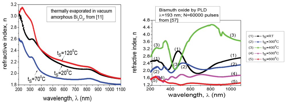
Figure 12. Wavelength dependence of the refractive index for different types of bismuth oxide films [11, 57].
