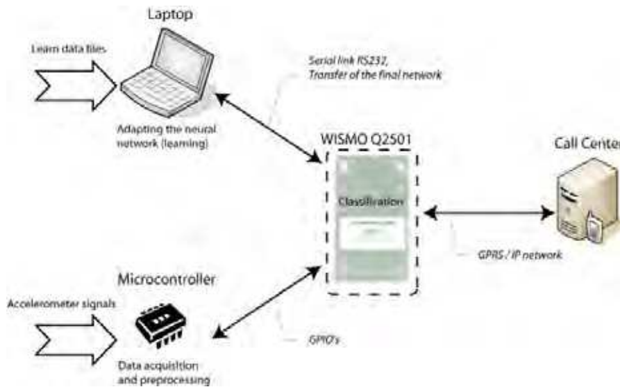
Figure 13. Hardware architecture
