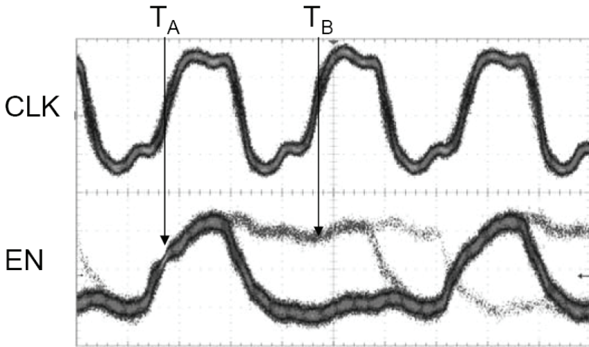
Figure 10. Accumulative display of synchronized EN signal with finite probability of delayed synchronization
