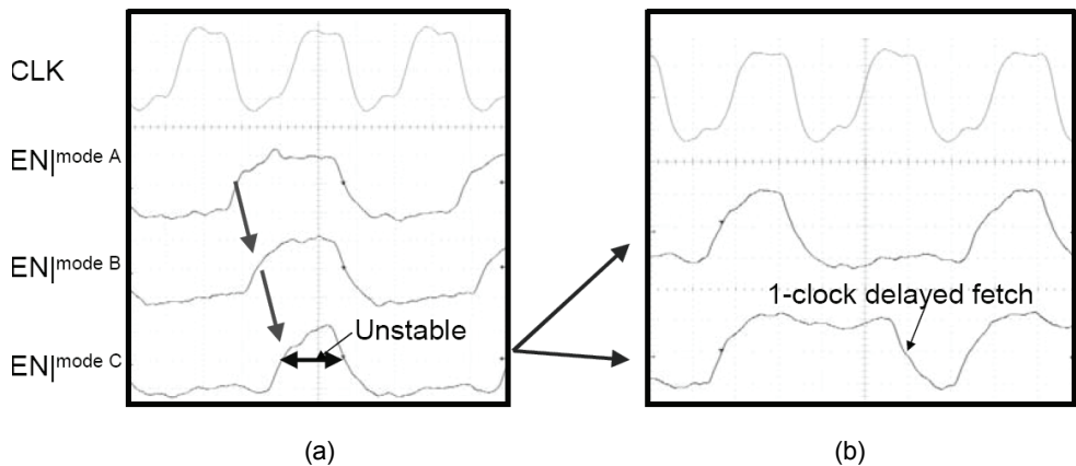
Figure 9. Uncertainty in non-synchronized global interconnect
