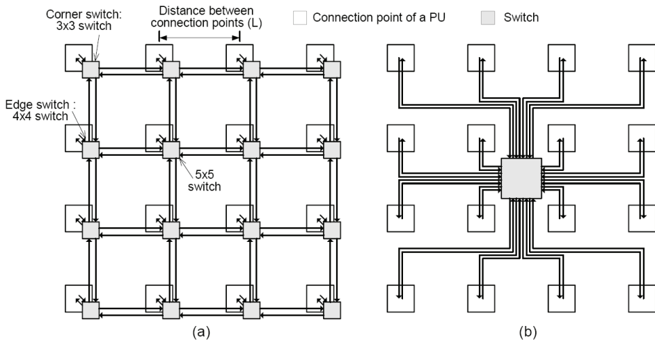
Figure 3. (a) Mesh and (b) Start topology configurations
