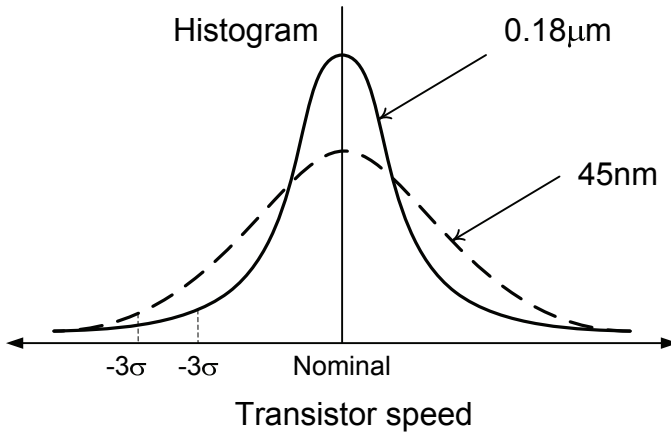
Figure 1. Distribution of transistor characteristics for different feature sizes
