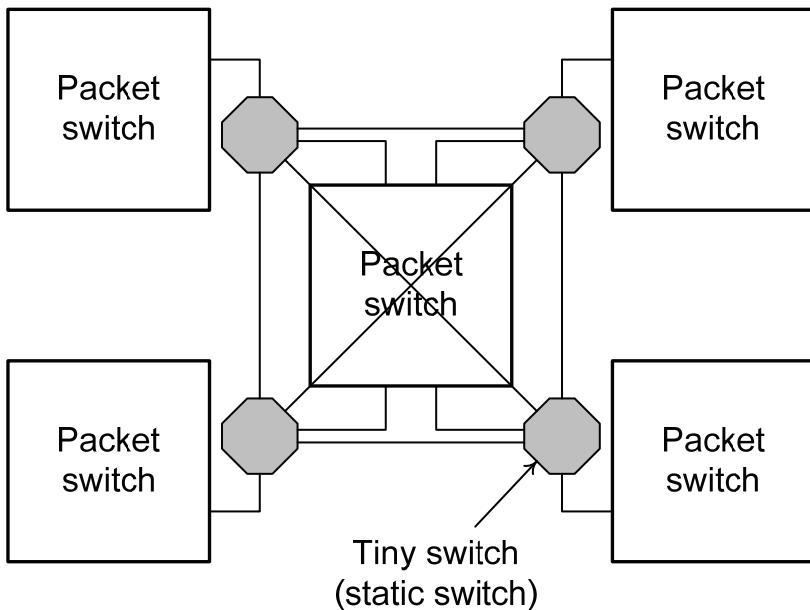
Figure 4. Configurable network topology with tiny switches
