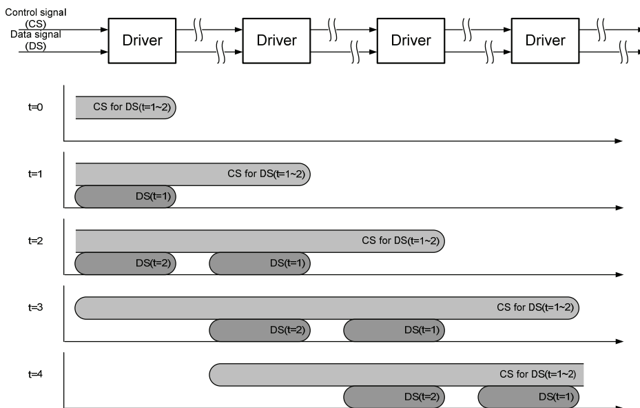
Figure 7. Wave-pipelining scheme for the control signal
