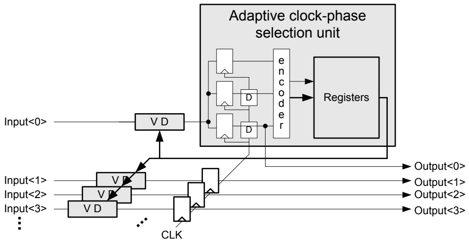
Figure 8. Adaptive clock-phase selection with variable delay circuit
