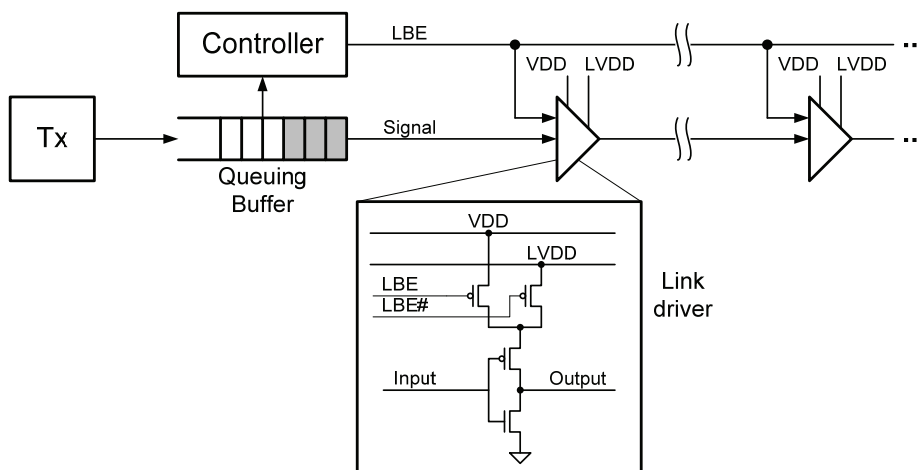
Figure 6. Adaptive bandwidth adjustment circuit
