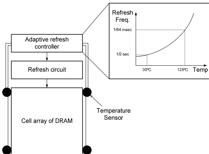
Figure 2. An example of DRAM block diagram with adaptive refresh scheme
