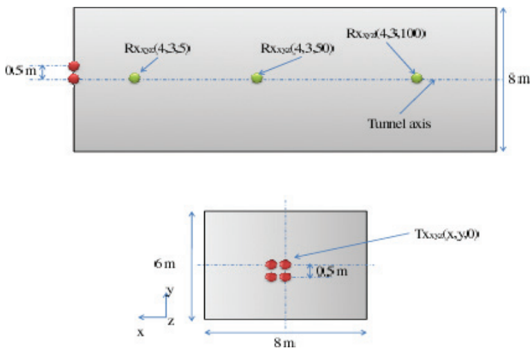
Figure 7. Time focusing simulation setup.
