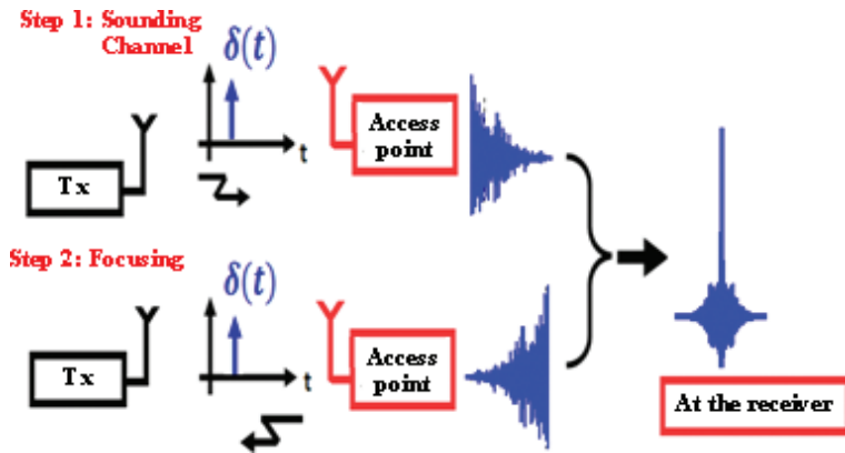
Figure 5. Principle of time reversal technique.
