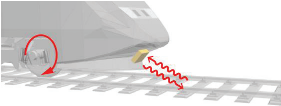
Figure 2. Proprioceptive sensors to feed the train odometer.
