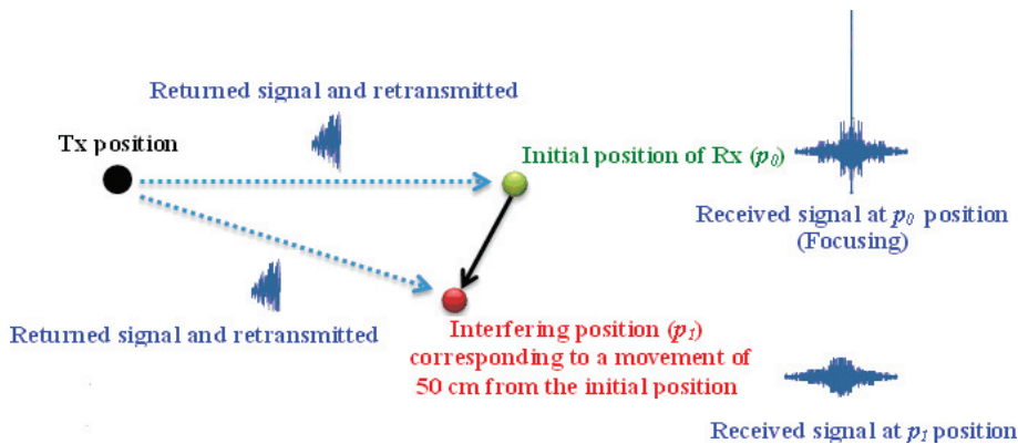
Figure 11. Principle of SF measurement.
