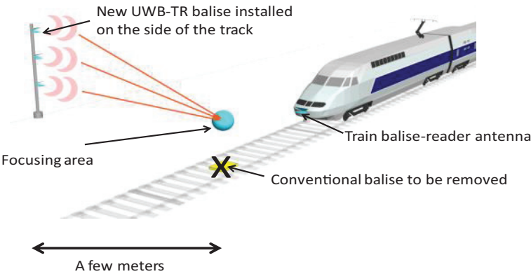
Figure 4. The new proposed railway balise.
