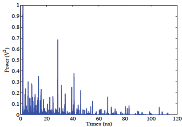
Figure 6. Averaged and normalised power delay profile (PDP).
