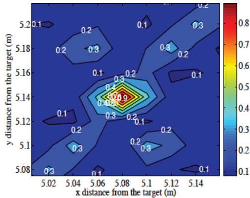
Figure 9. Spatial focusing gain in the SISO-TR case.
