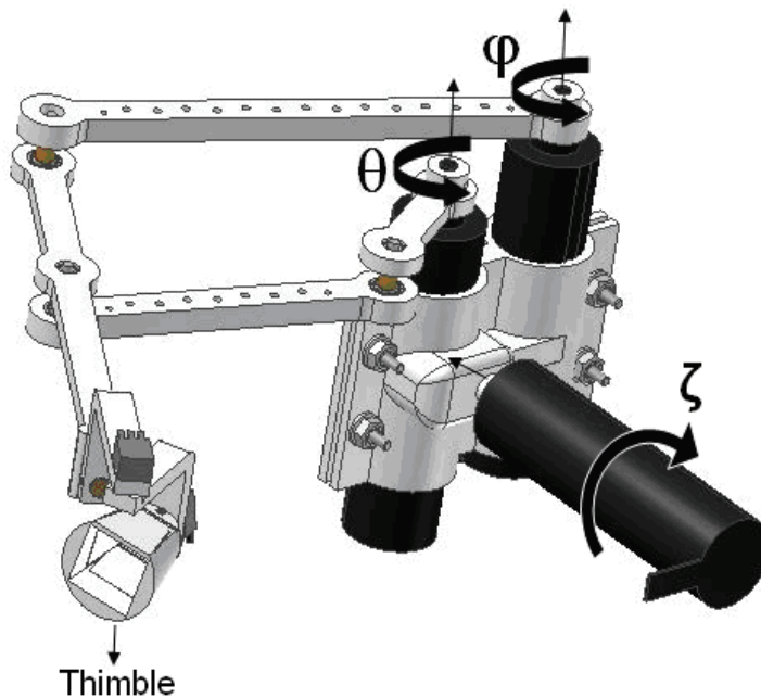
Fig. 1. Design of MasterFinger Modules
