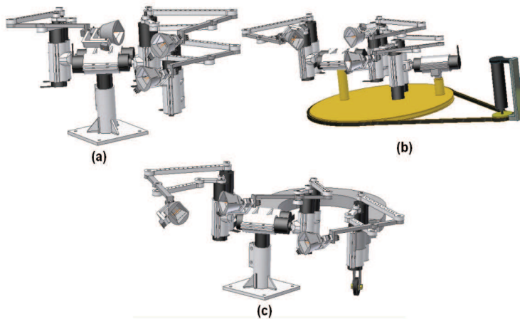
Fig. 6. Three different Masterfinger-3 designs
