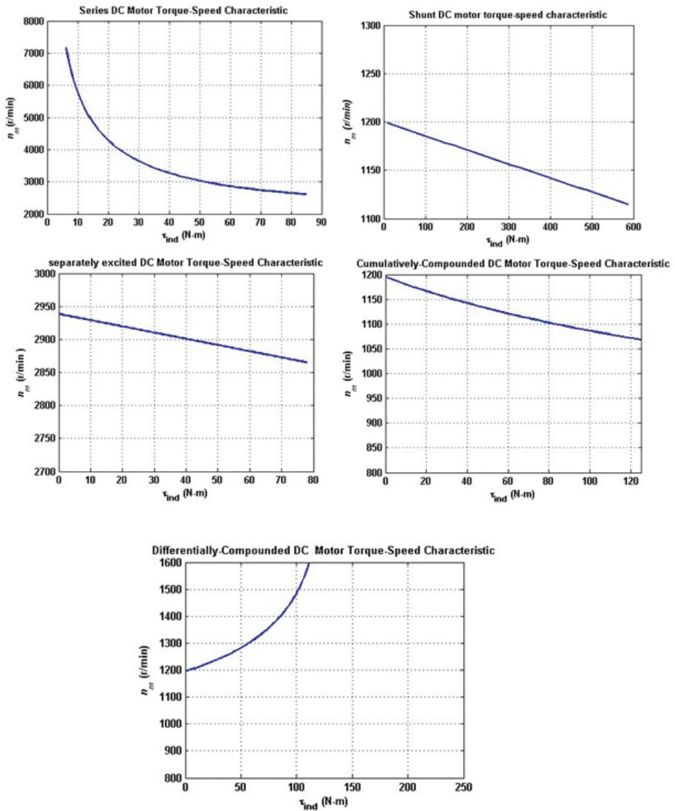
Figure 14. DC motor terminal characteristics.
