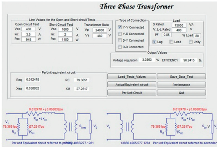
Figure 11. Per unit equivalent circuit of three-phase transformer.
