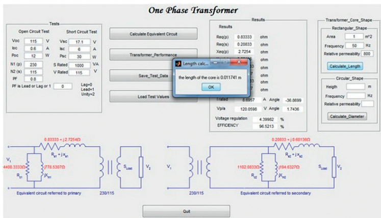
Figure 8. Transformer core shape calculated.
