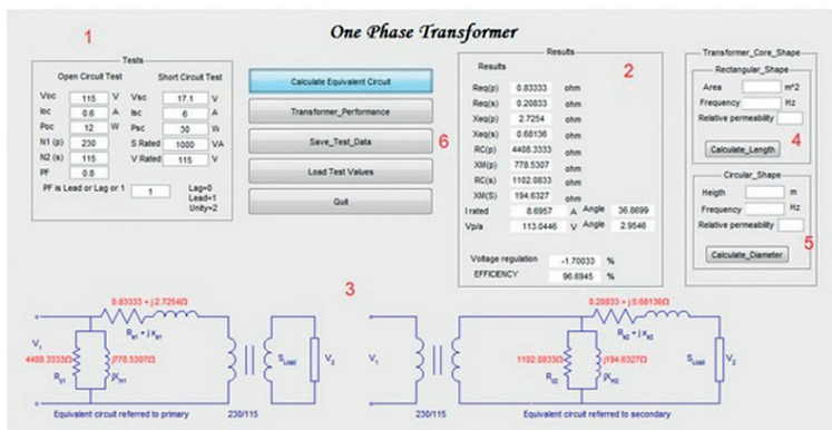
Figure 7. Graphical user interface for single-phase transformer.
