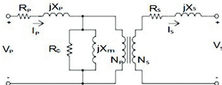
Figure 5. Exact model of transformer.
