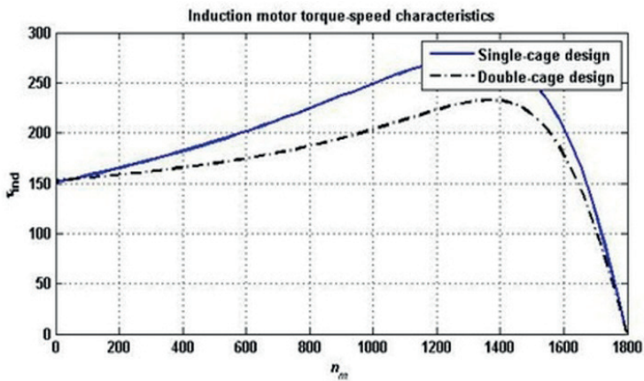
Figure 20. Single- and double-cage rotor characteristic.
