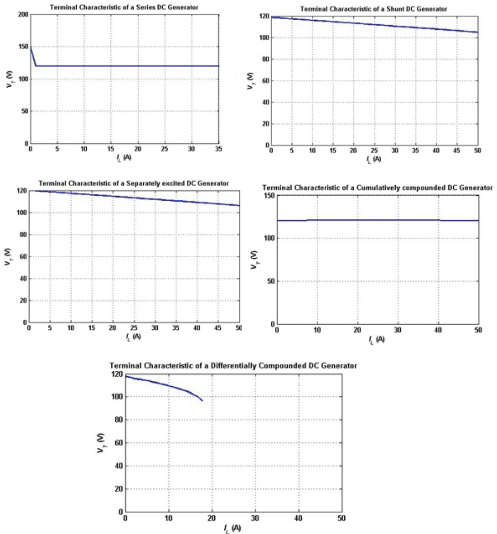
Figure 15. DC generator terminal characteristics.
