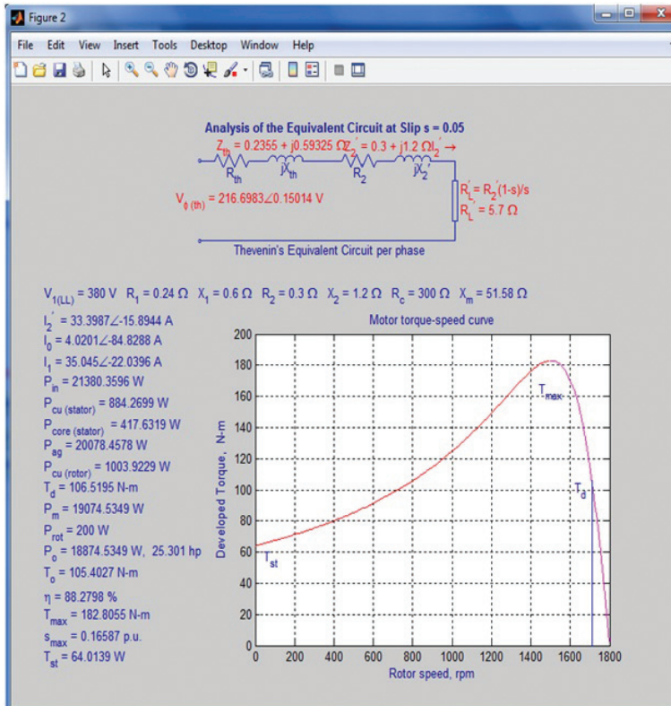
Figure 19. Equivalent circuit and torque speed characteristic.
