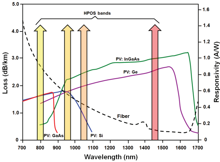
Figure 2. Qualitative graph of some PoF parameters.
