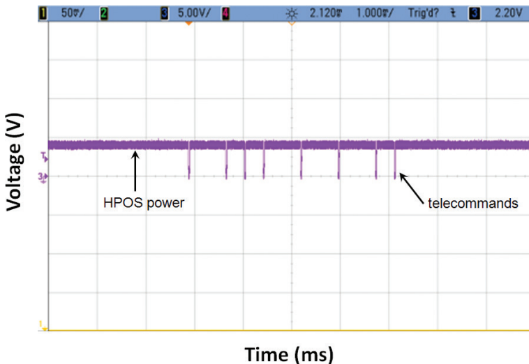
Figure 3. Oscilloscope trace showing a telecommand signal transmitted over the optical supply power.
