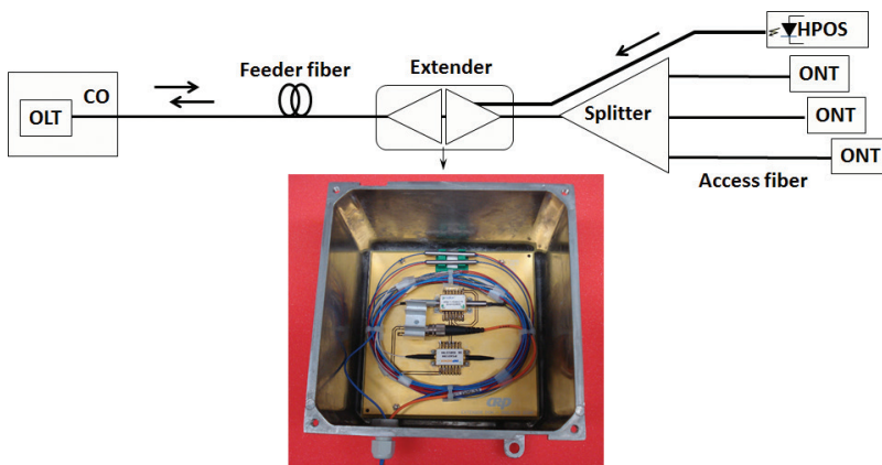
Figure 9. Schematic of a PON using extender powered by a PoF system and the extender photo.
