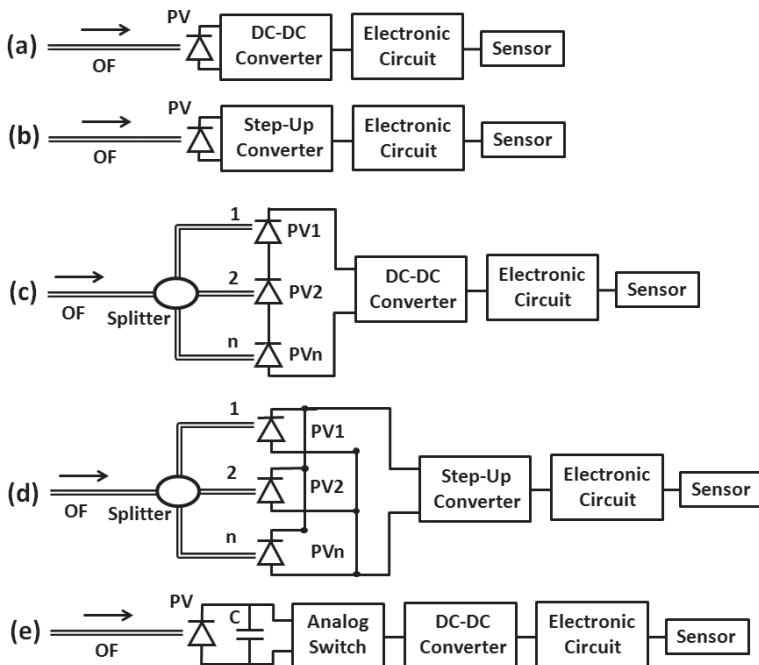
Figure 6. Some types of circuits used in the design of PoF remote units, (a) direct conversion, (b) conversion using a step-up converter, (c) PVs connected in series, (d) PVs connected in parallel, and (e) charging circuit using a capacitor.
