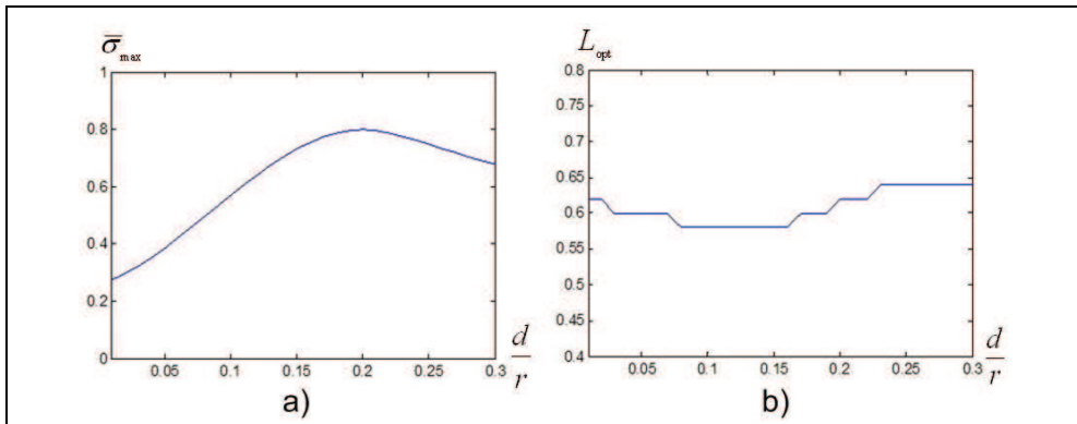
Fig. 6. The plots of a) \bar{\sigma}_{max} and b) L_{opt} , for 0 < d \leq 0.3
