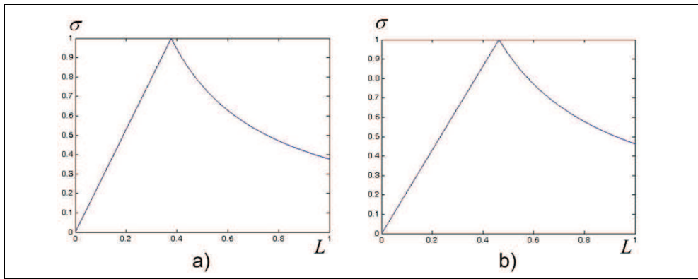
Fig. 4. The plots of \sigma(\theta_{iso}) for 0 < L \leq 1.0 : a) SM1 and b) SM3
