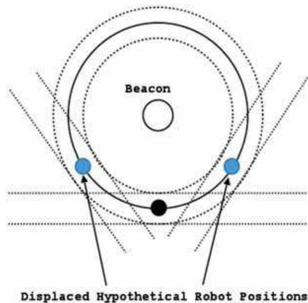
Fig. 7. Our system adds low weight Gaussians rotated around the beacon, meaning we linearise around multiple points
