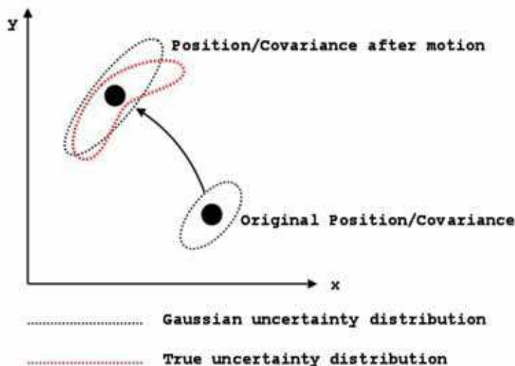
Fig. 2. Gaussian approximation to a non-linear motion update
